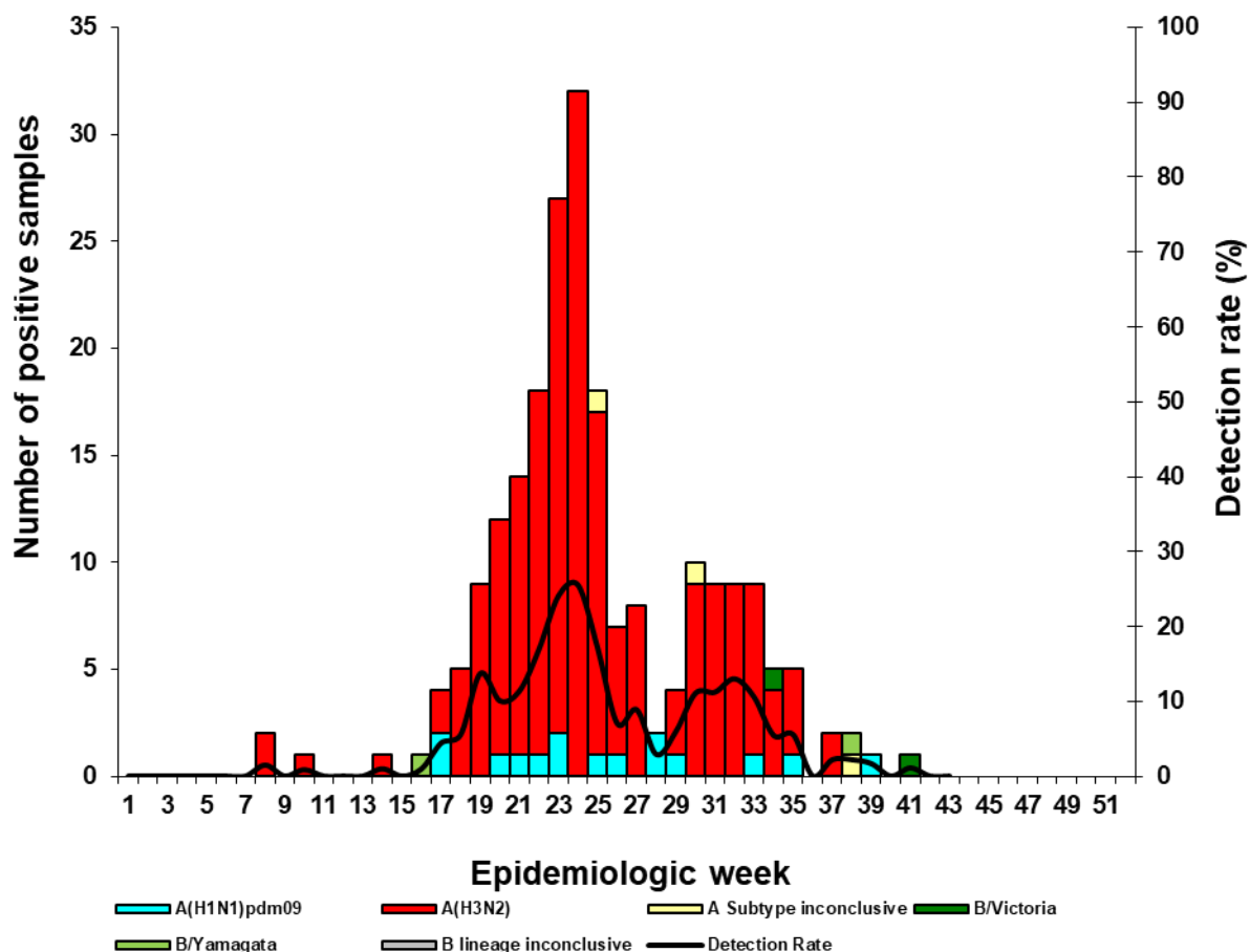
Figure 5. Number of positive samples* by influenza subtype and lineage and detection rate** by week
