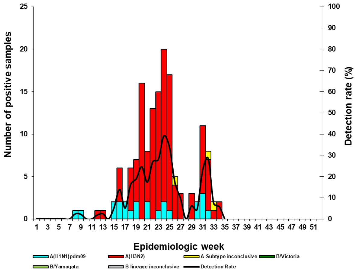
Figure 1. Number of positive samples* by influenza subtype and lineage and detection rate** by week
