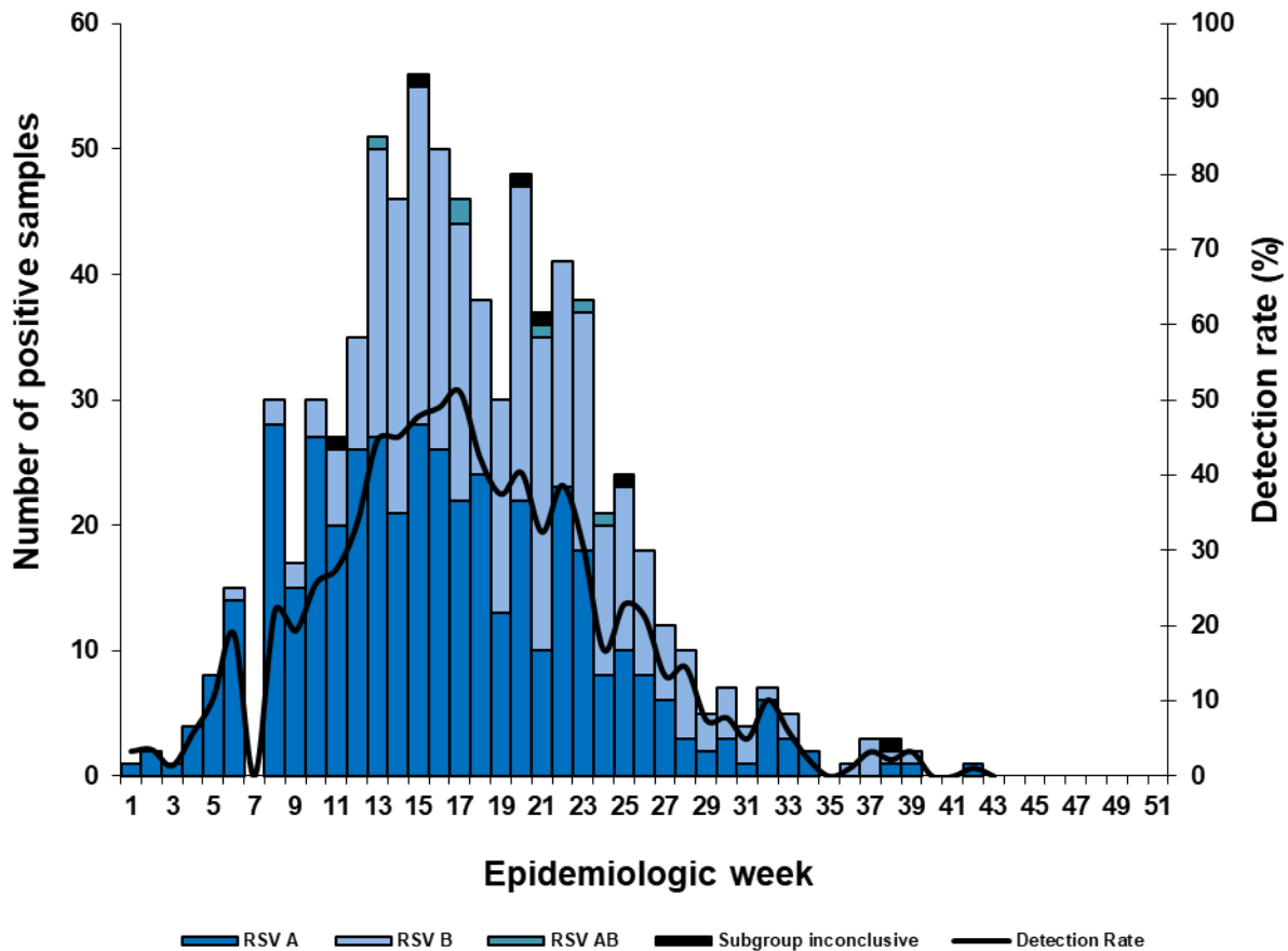
Figure 6. Number of samples testing positive for respiratory syncytial virus by subgroup and detection rate by week
