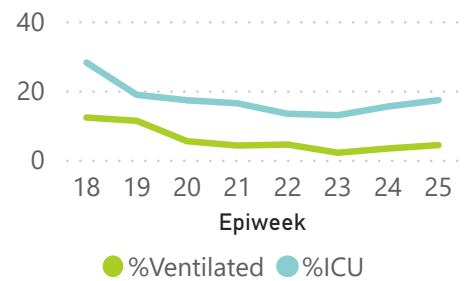
%ICU and %Ventilated per week Gauteng Total: 1334
