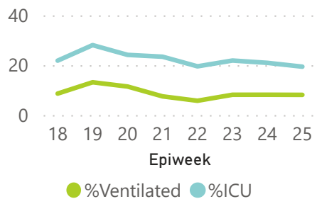
%ICU and %Ventilated per week Eastern Cape Total: 777
