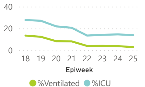
%ICU and %Ventilated per week KwaZulu Natal Total: 633
