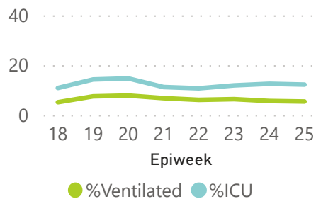
%ICU and %Ventilated per week Western Cape Total: 6390
