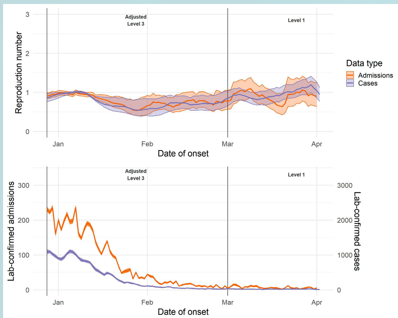
Figure 6. Upper panel: Estimated daily reproduction number (R), with 95% confidence intervals, Eastern Cape (last date included in the estimation: 01 April 2021). Lower panel: estimated number of laboratory-confirmed COVID-19 cases and hospital admissions by onset date with missing data imputed. The medians and 95% ranges for the imputed datasets are shown. Daily numbers of confirmed laboratory-confirmed COVID-19 cases in the bottom panel are shown on the right-hand y axis.
