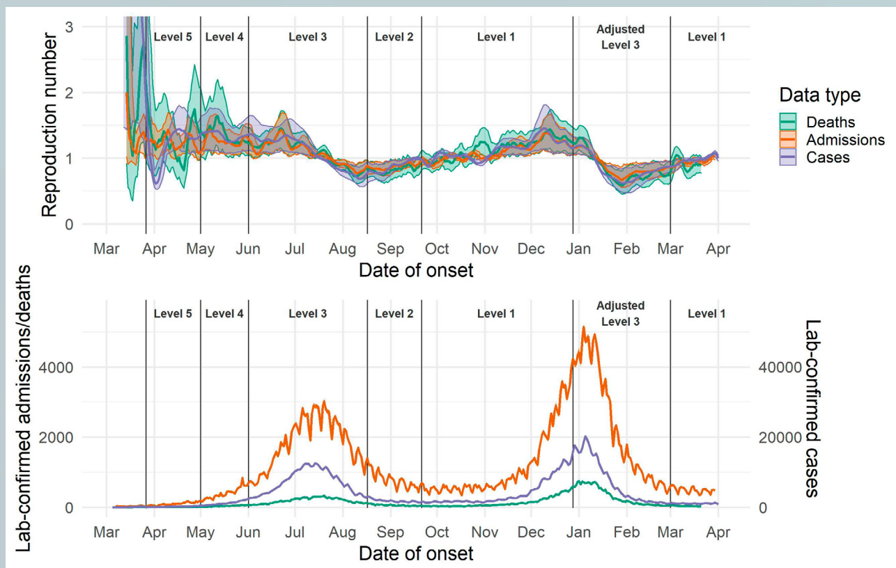
Figure 2. Upper panel: Estimated daily reproduction number (R), with 95% confidence intervals, South Africa (last date included in the estimation: 01 April). Lower panel: estimated number of laboratory-confirmed COVID-19 cases, hospital admissions, and deaths, by onset date with missing data imputed. The medians and 95% ranges for the imputed datasets are shown. Daily numbers of confirmed laboratory-confirmed COVID-19 cases in the bottom panel are shown on the right-hand y axis.
