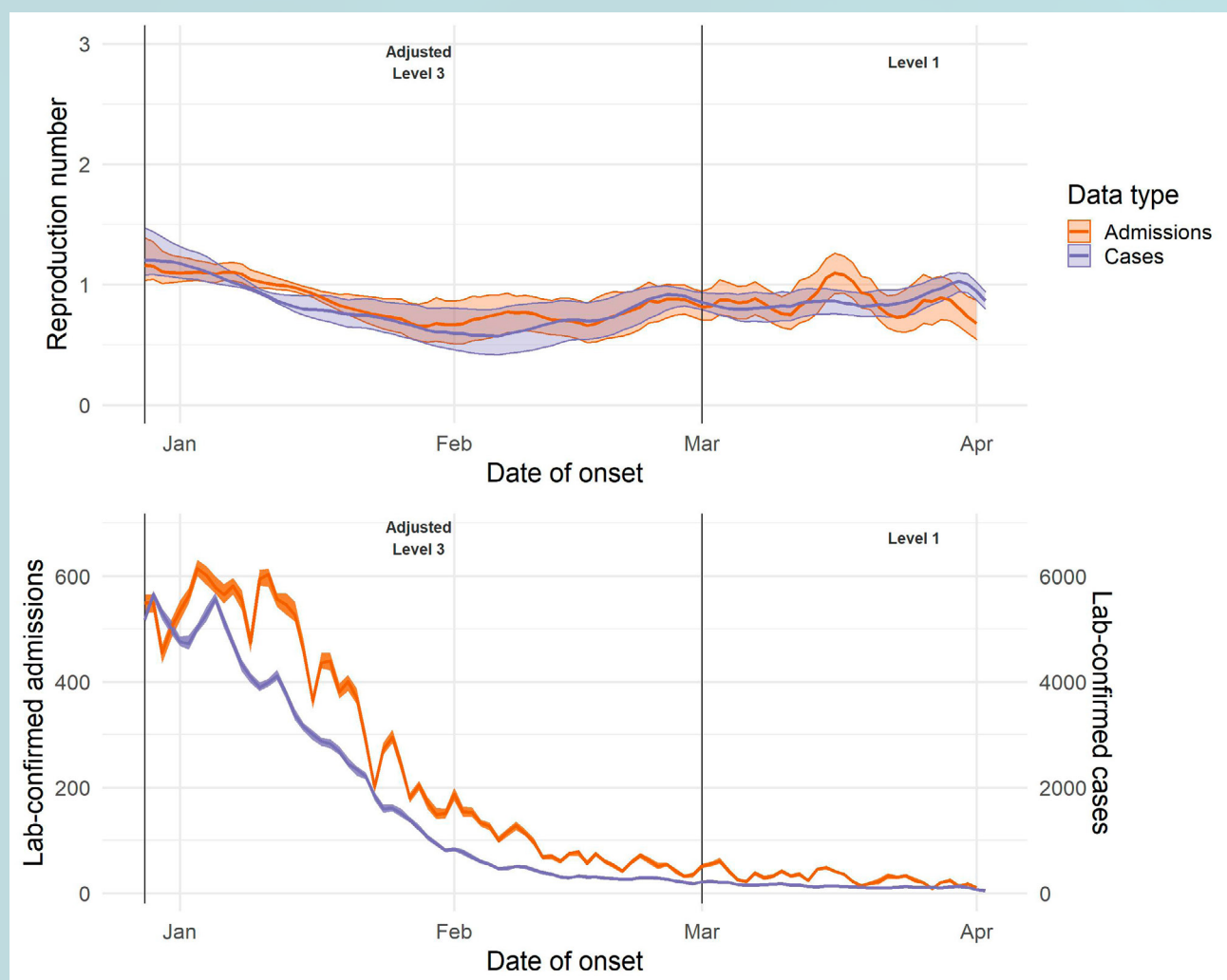
Figure 7. Upper panel: Estimated daily reproduction number (R), with 95% confidence intervals, KwaZulu-Natal (last date included in the estimation: 01 April 2021). Lower panel: estimated number of laboratory-confirmed COVID-19 cases and hospital admissions by onset date with missing data imputed. The medians and 95% ranges for the imputed datasets are shown. Daily numbers of confirmed laboratory-confirmed COVID-19 cases in the bottom panel are shown on the right-hand y axis.
