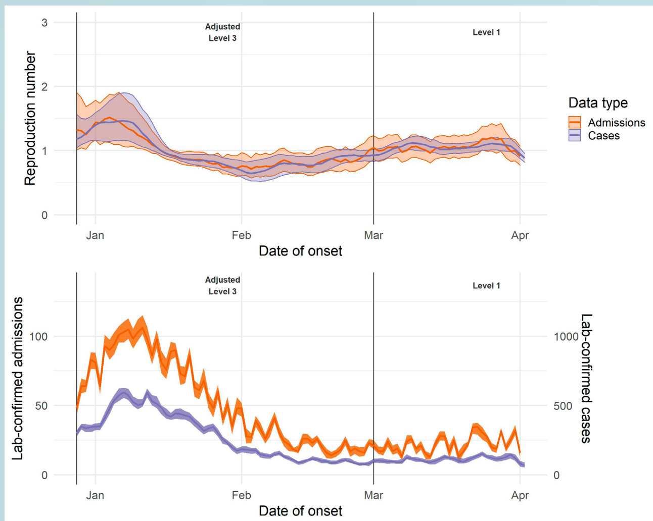
Figure 8. Upper panel: Estimated daily reproduction number (R), with 95% confidence intervals, Free State (last date included in the estimation: 01 April 2021). Lower panel: estimated number of laboratory-confirmed COVID-19 cases and hospital admissions by onset date with missing data imputed. The medians and 95% ranges for the imputed datasets are shown. Daily numbers of confirmed laboratory-confirmed COVID-19 cases in the bottom panel are shown on the right-hand y axis.
