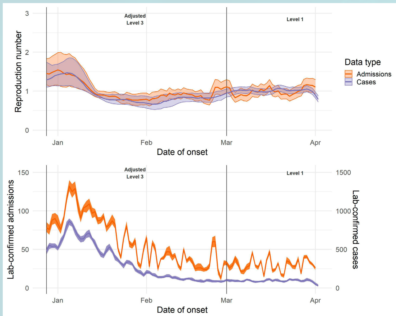
Figure 10. Upper panel: Estimated daily reproduction number (R), with 95% confidence intervals, North West (last date included in the estimation: 01 April 2021). Lower panel: estimated number of laboratory-confirmed COVID-19 cases and hospital admissions by onset date with missing data imputed. The medians and 95% ranges for the imputed datasets are shown. Daily numbers of confirmed laboratory-confirmed COVID-19 cases in the bottom panel are shown on the right-hand y axis.
