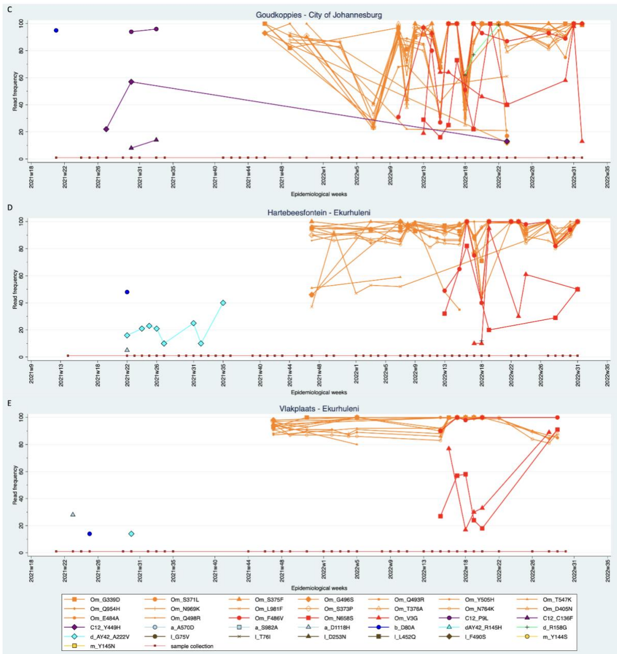
Figure 1: Beta mutation (D80A, dark blue circle). Delta mutations: R145H (pale blue triangle), R158 (green cross), A222V (pale blue diamond). C.1.2 mutations: P9L (purple circle), C136F (purple triangle), Y449H purple diamond. Omicron mutations: G339D (orange square), S371L (orange circle), S375F (orange triangle), G496S (orange diamond), Q493R (orange dot), Y505H (medium point orange circle), T547K (orange small triangle), Q954H (orange small diamond), N969K (orange small line), L981F (orange small x), S373P (orange hollow diamond), T376A (orange hollow triangle), D405N (small orange hollow triangle), E484A (small orange solid circle), Q498R (point orange circle), F486V (red circle), N658S (red square) and V3G (red triangle). Dots on the red line shows the timepoints of sample collection, absence of specific coloured lines means the mutation was not detected at that timepoint. A (Rooiwal plant), B (Daspoort plant), C (Goudkoppies plant), D (Hartebeesfontein plant), and E (Vlakplaats plant).
