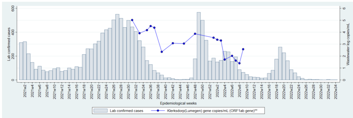
Figures 7A-7C. Laboratory confirmed cases of SARS-CoV-2 (bars) and levels of SARS-CoV-2 in log copies/ml of wastewater (coloured lines) in wastewater treatment plants (WWTPs) from Potchefstroom, JB Marks District (A) Rustenburg, Bojanala District (B), and City of Matlosana, Northwest Province during epidemiological weeks 1, 2021 to 34, 2022. The testing laboratory and quantified SARS-CoV-2 gene are named in brackets after the name of the WWTP. Note that comparisons of levels over time should only be made for specimens tested in the same laboratory.
