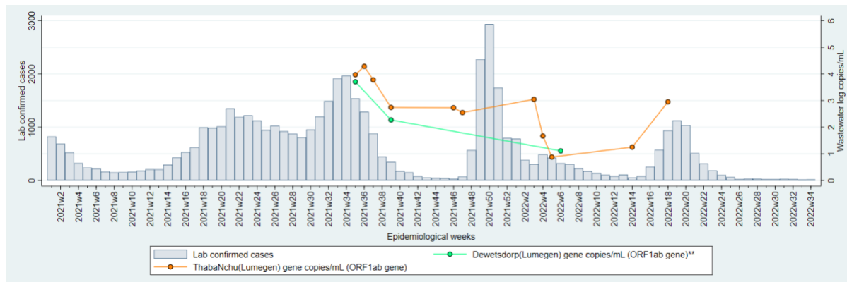
Figures 3A-C. Laboratory confirmed cases of SARS-CoV-2 (bars) and levels of SARS-CoV-2 in log copies/ml of wastewater (coloured lines) from wastewater treatment plants (WWTPs) in Mangaung, Free State Province (Bloemfontein, Botshabelo, Naledi and ThabaNchu) during epidemiological weeks 1, 2021 to 34, 2022. The testing laboratory and quantified SARS-CoV-2 gene are named in brackets after the name of the WWTP. Note that comparisons of levels over time should only be made for specimens tested in the same laboratory.
