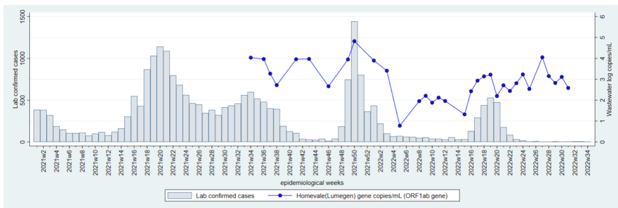
Figures 6A-B. Laboratory confirmed cases of SARS-CoV-2 (bars) and levels of SARS-CoV-2 in log copies/ml of wastewater (coloured lines) in wastewater treatment plants (WWTPs) from Calvinia in Namakwa Metro (a) and Kimberly in Frances Baard District (b), Northern Cape Province during epidemiological weeks 1, 2021 to week 34, 2022. The testing laboratory and quantified SARS-CoV-2 gene are named in brackets after the name of the WWTP. Note that comparisons of levels over time should only be made for specimens tested in the same laboratory.
