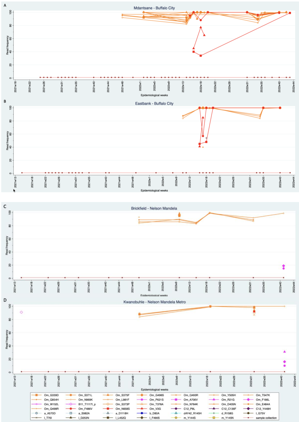
Figure 5: Beta mutation (D80A, dark blue circle). Delta mutations: R145H (pale blue triangle), E156del (green square), R158 (green cross), A222V (pale blue diamond). C.1.2 mutations: P9L (purple circle),
