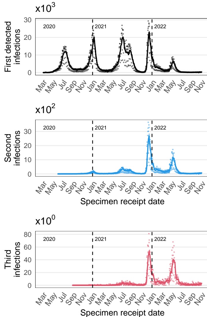
Figure 1: Daily numbers of detected primary infections and suspected reinfections in South Africa. (Top) Time series of first detected (primary) infections. (Middle) Time series of suspected second infections. (Bottom) Time series of suspected third infections. Lines indicate 7-day moving average; points are daily values.
