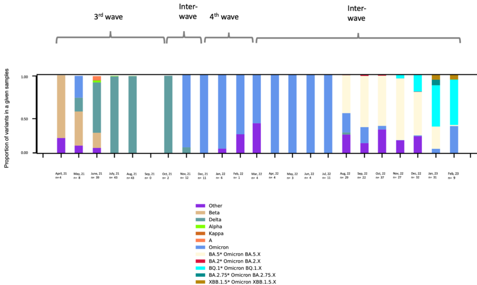
Figure 1. The proportion of SARS-CoV-2 variants in the environmental samples sorted by month and year (April 2021-February, 2023) from all South African provinces. The number of samples processed each month, with a coverage >50% are indicated as n.
