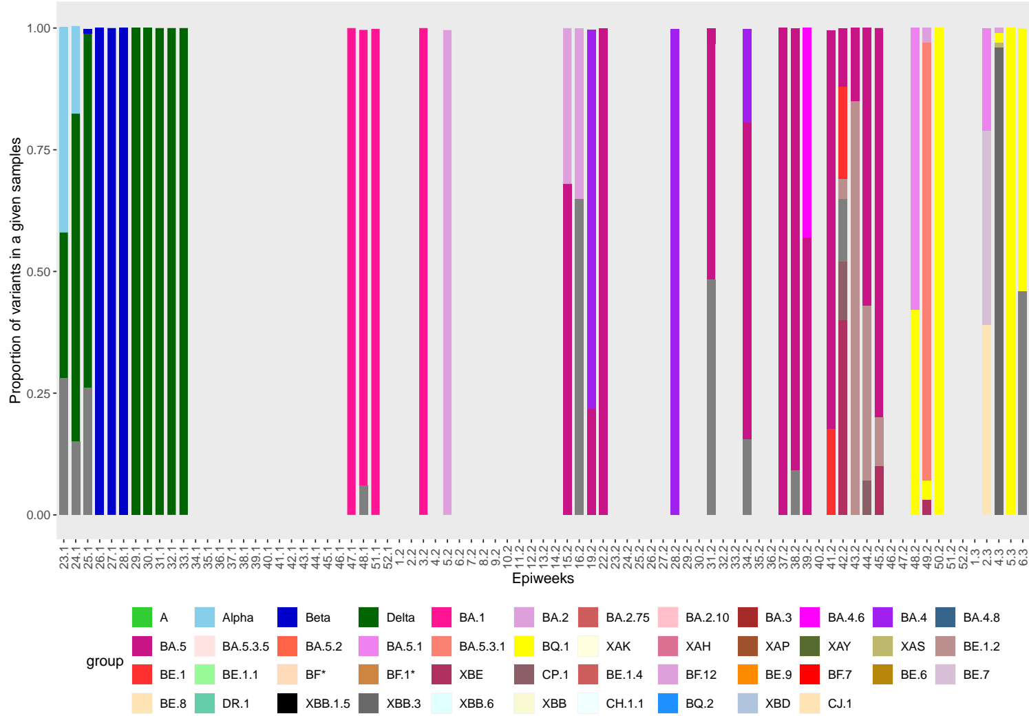
Figure 5: The proportion of SARS-CoV-2 variants and lineages in the environmental samples collected from Vlakplaats, in the Ekurhuleni region, arranged chronologically by epidemiological week (i.e. 22.1 is epidemiological 22, year 2021). Only samples that had a coverage of >50% were included in the analysis.
