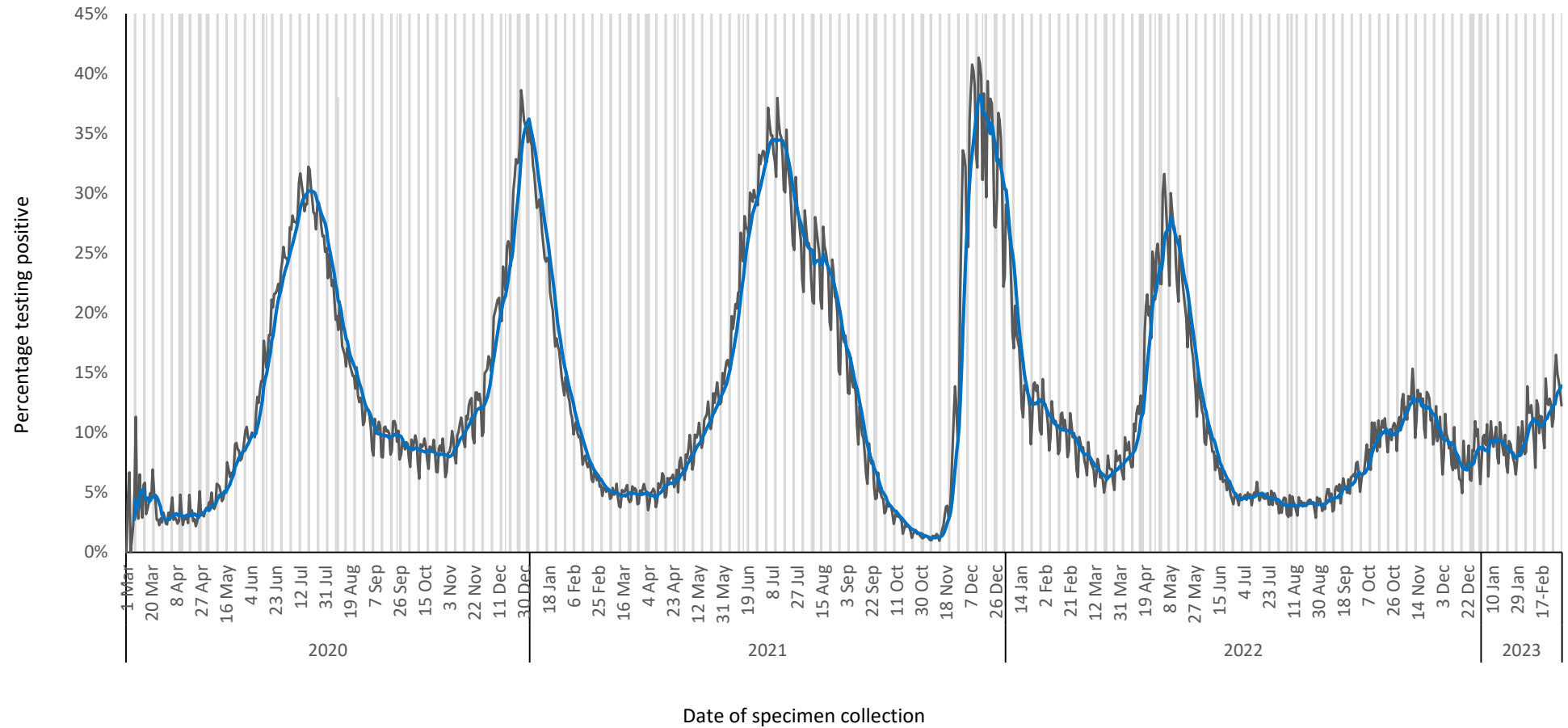
Figure 3. Percentage of PCR tests positive for SARS-CoV-2 by date of specimen collection, South Africa, 1 March 2020 – 4 March 2023. Blue line shows the 7-day moving average of the percentage testing positive. Grey bars highlight weekend days and public holidays.
