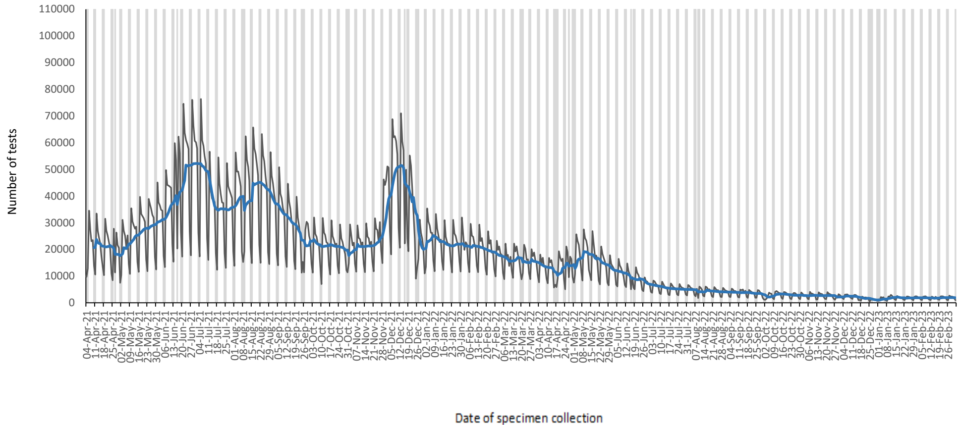
Figure 1. Number of SARS-CoV-2 PCR tests reported by date of specimen collection, South Africa, 4 April 2021 – 4 March 2023. Blue line shows the 7-day moving average of the number of PCR tests reported. Grey bars highlight weekend days and public holidays.
