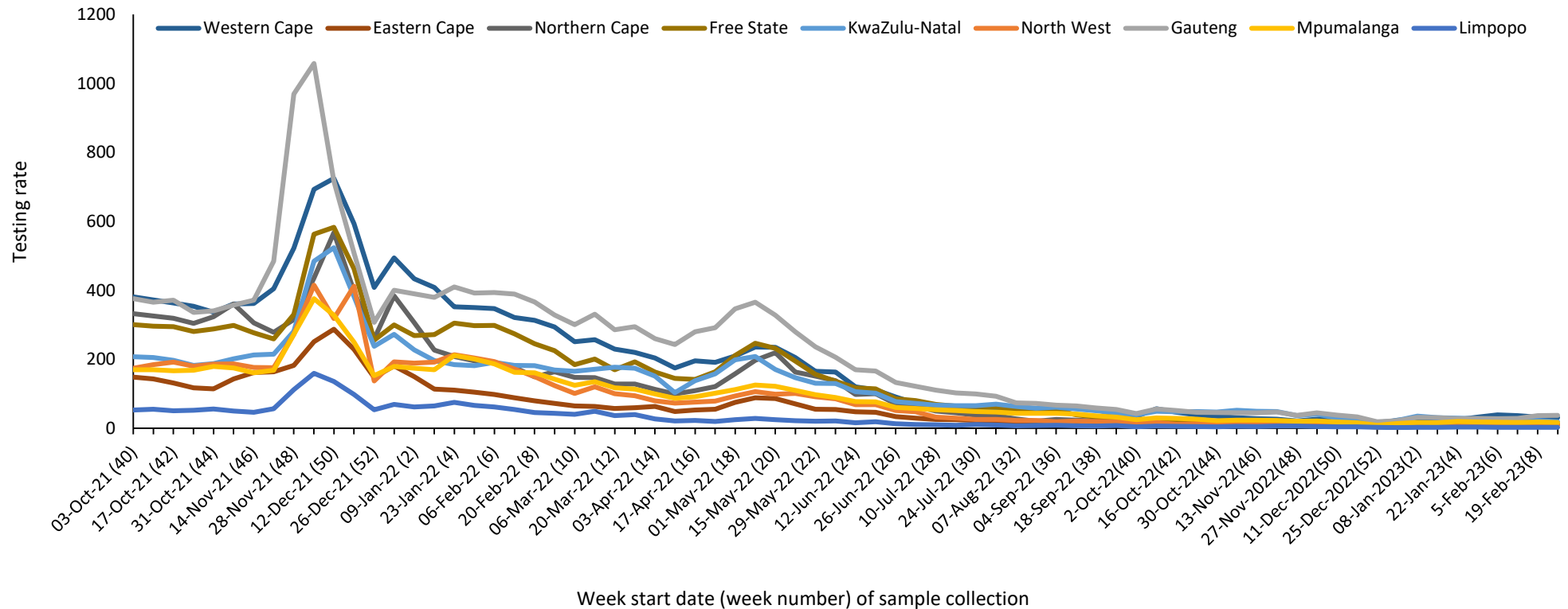
Figure 2. PCR testing rate per 100,000 persons by province and week of specimen collection, South Africa, 3 October 2021 – 4 March 2023
