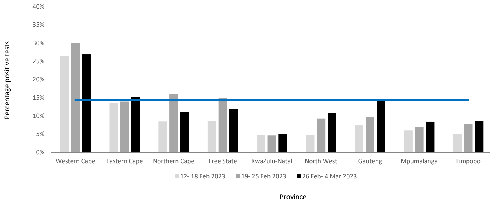
Figure 4. Weekly percentage testing positive (PCR tests only) by province, South Africa, 12 February 2023 – 4 March 2023. The horizontal blue line shows the national mean for week 9, beginning 26 February 2023
