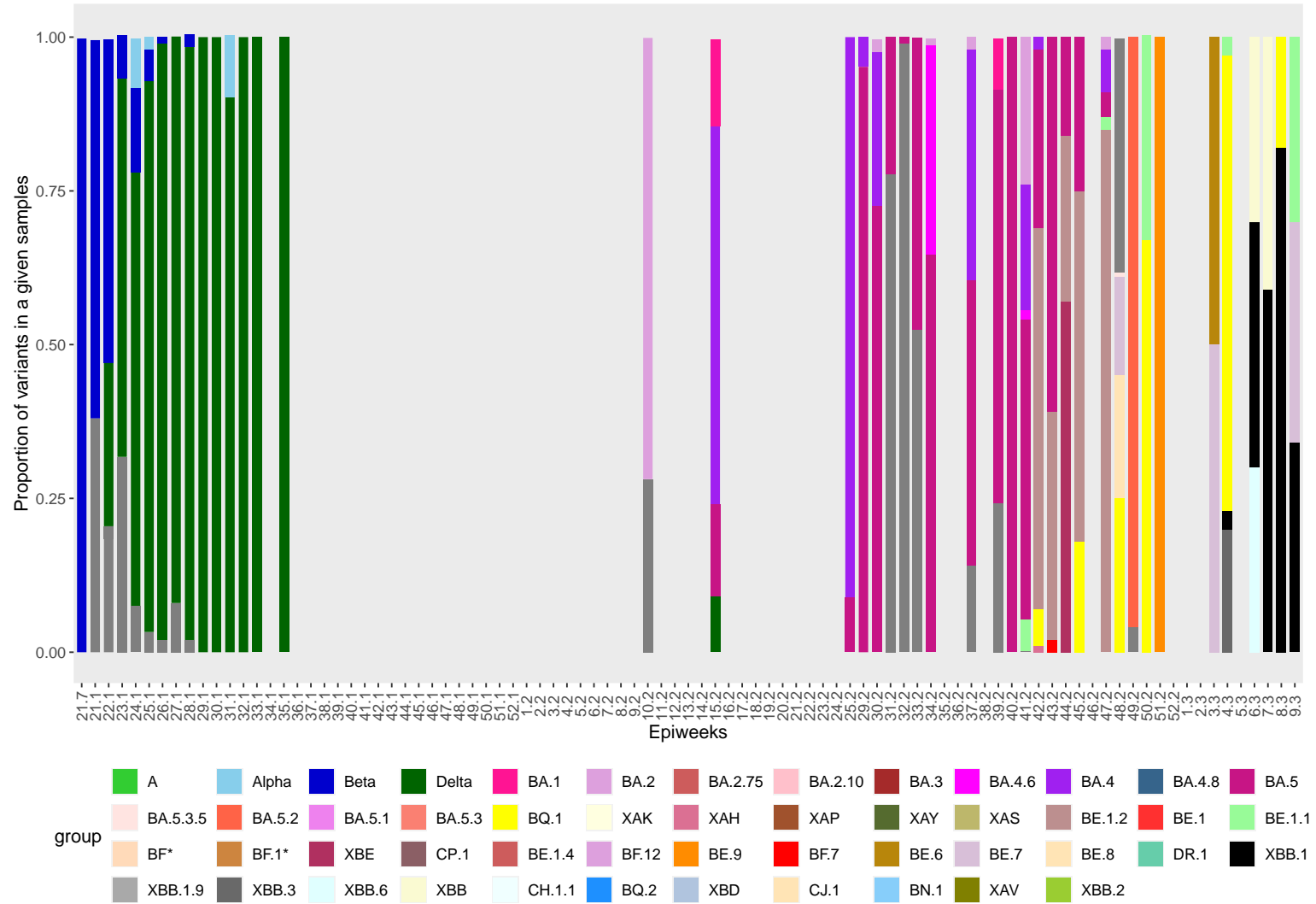
Figure 4: The proportion of SARS-CoV-2 variants and lineages in the environmental samples collected from Rooiwal, in the Tshwane region, arranged chronologically by epidemiological week (i.e. 22.1 is epidemiological 22, year 2021). Only samples that had a coverage of >50% were included in the analysis.
