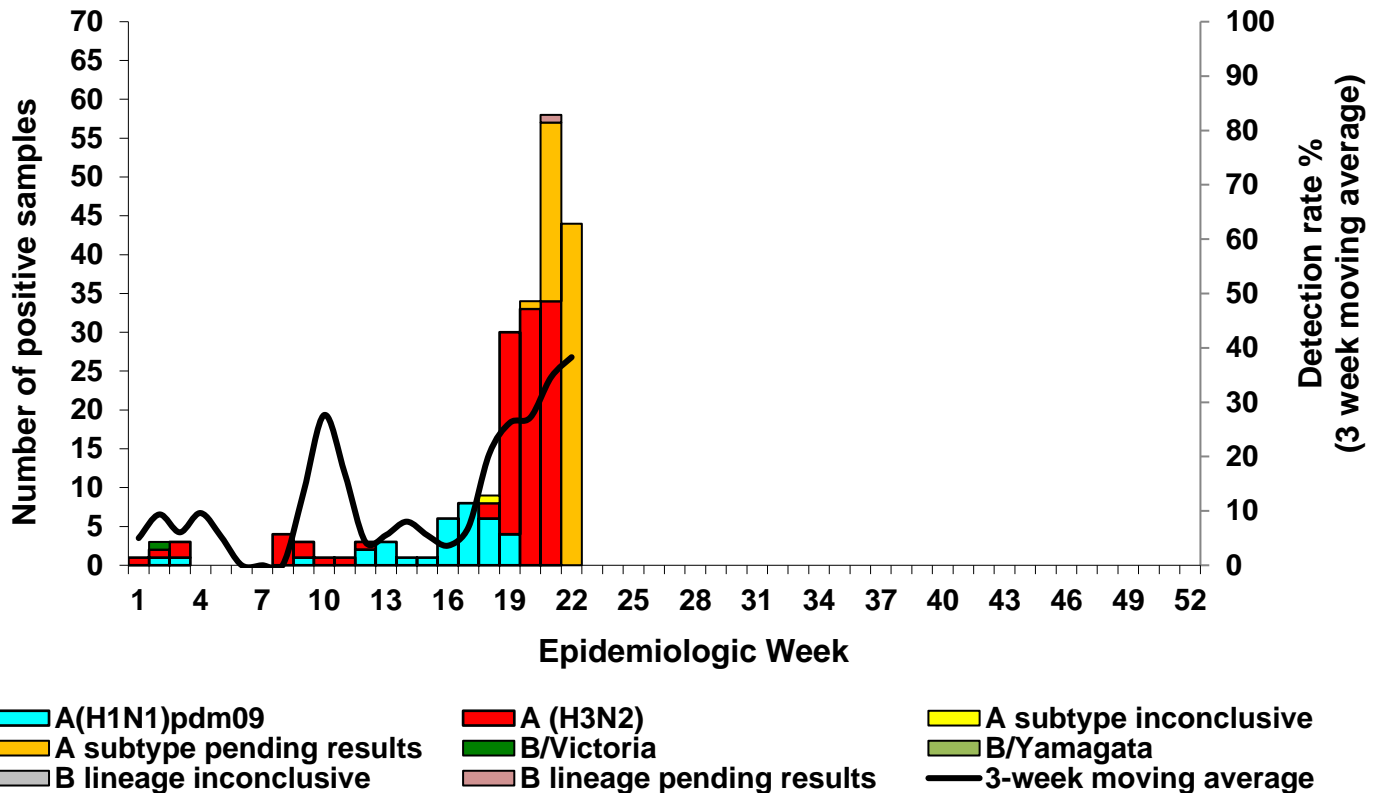
Figure 8. Number of positive patients* by influenza subtype and lineage and 3-week moving average by week, ILI surveillance - Viral Watch, 01/01/2023-04/06/2023
