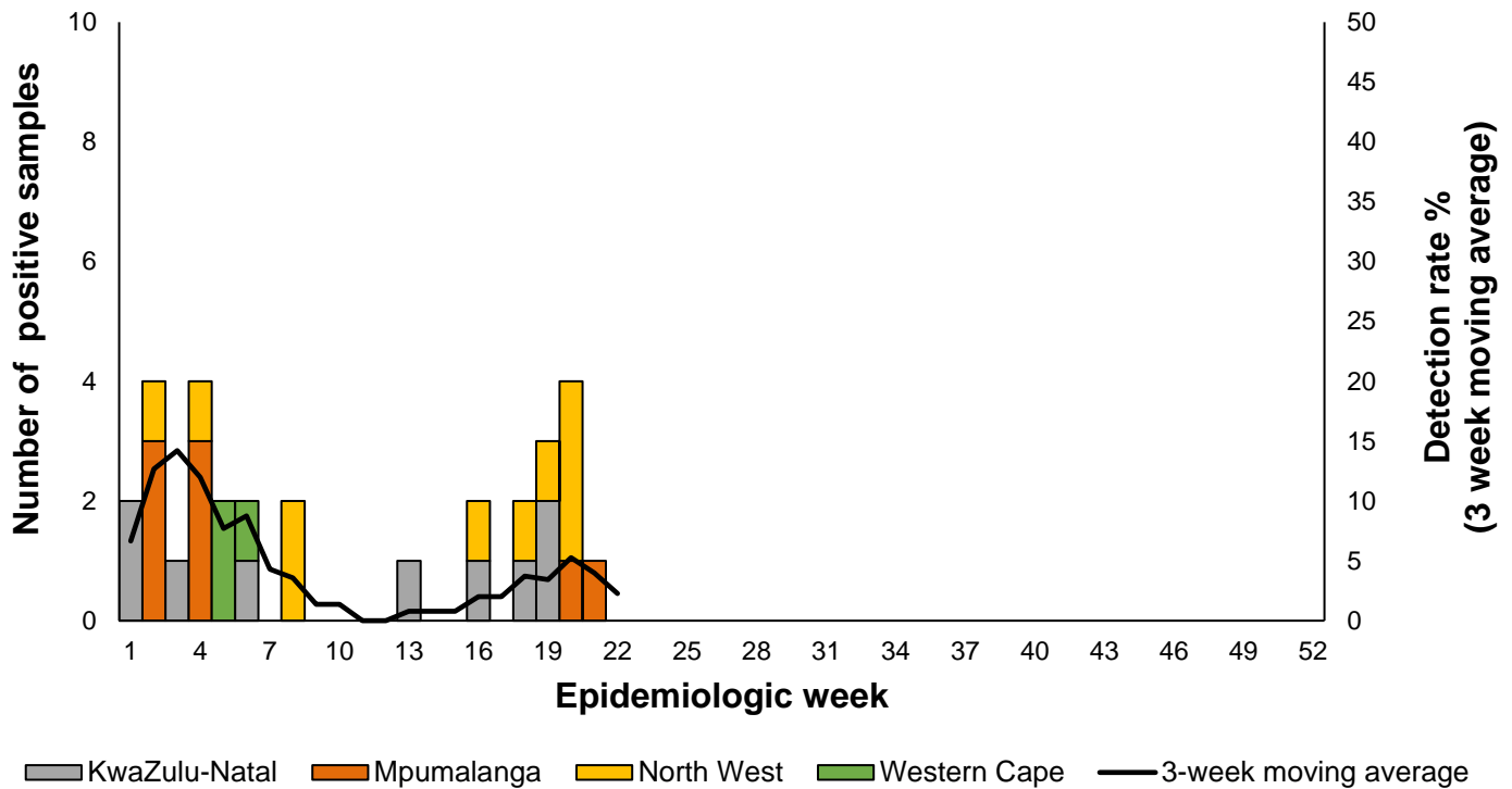
Figure 6. Number of patients* testing positive for SARS-CoV-2** by province and 3-week moving average by week, influenza-like illness (ILI) surveillance in primary health care clinics, 01/01/2023 –04/06/2023
