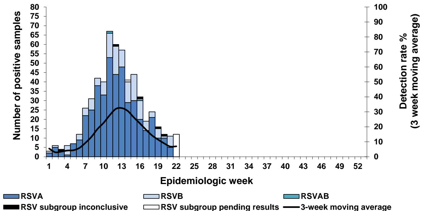
Figure 15. Number of patients (all ages) testing positive for respiratory syncytial virus* by subgroup and 3-week moving average by week, pneumonia surveillance public hospitals, 01/01/2023-04/06/2023
