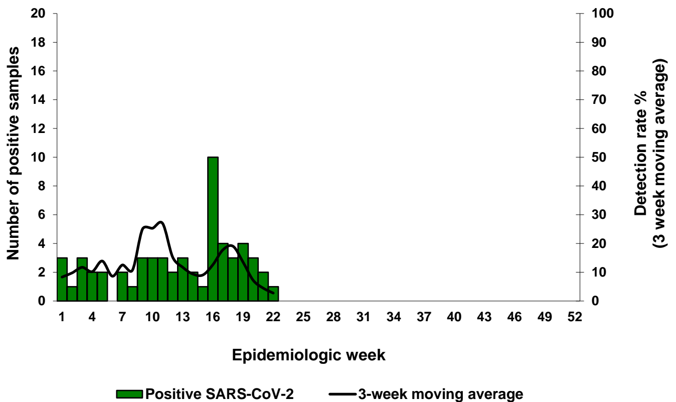
Figure 10. Number of patients testing positive for SARS-CoV-2*, by site and 3-week moving average** by week, ILI surveillance - Viral Watch, 01/01/2023-04/06/2023
