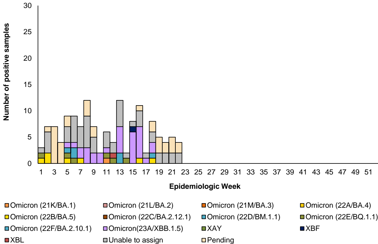
Figure 19. Number and 3-week moving average of laboratory-confirmed SARS-CoV-2 cases* by variant type (variant PCR/sequencing), pneumonia surveillance public hospitals, 01/01/2023-04/06/2023
