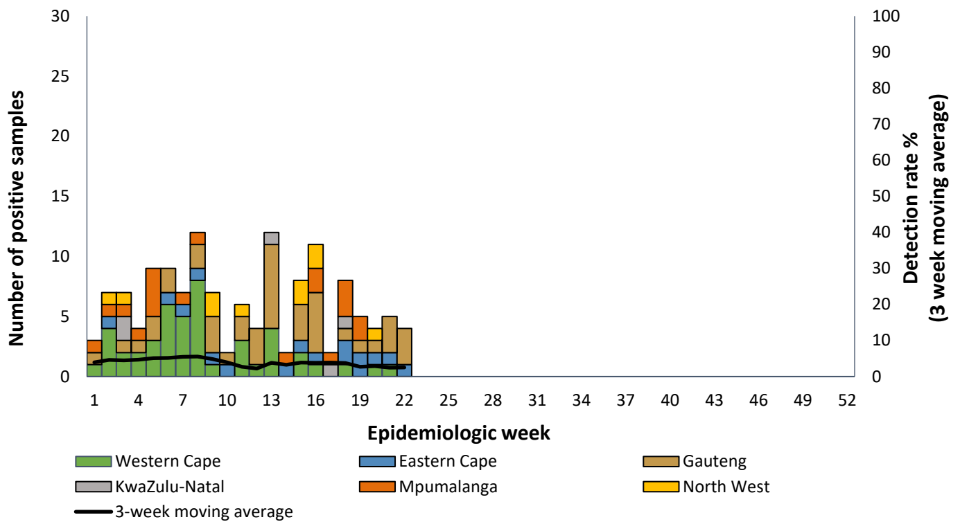
Figure 18. Number of patients testing positive for SARS-CoV-2** by province and 3-week moving average by week, pneumonia surveillance public hospitals, 01/01/2023-04/06/2023
