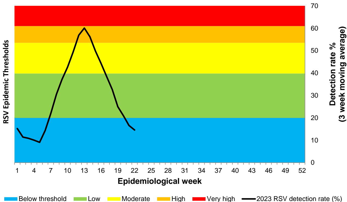
Figure 16. RSV percentage 3-week moving average and epidemic thresholds* among children aged < 5 years, pneumonia surveillance public hospitals, 01/01/2023-04/06/2023
