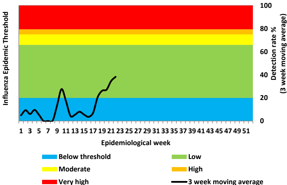
Figure 8b. Influenza percentage detections and epidemic thresholds* among cases of all ages, ILI surveillance - Viral Watch, 01/01/2023-04/06/2023
