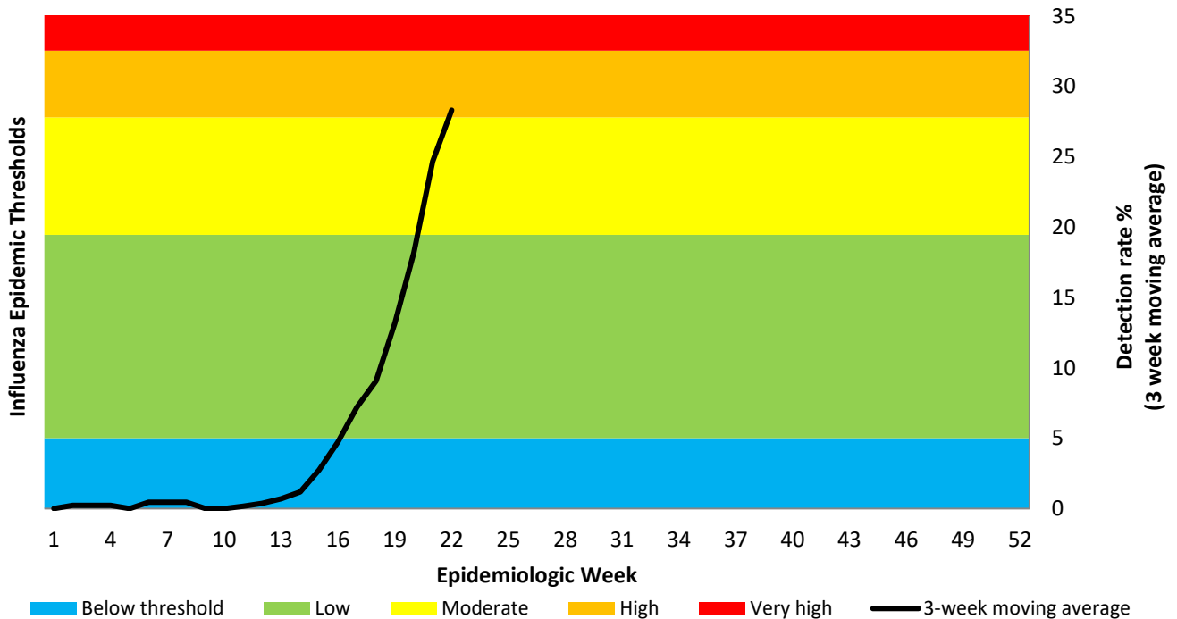
Figure 13. Influenza percentage detections and epidemic thresholds* among cases of all ages, pneumonia surveillance public hospitals, 01/01/2023-04/06/2023
