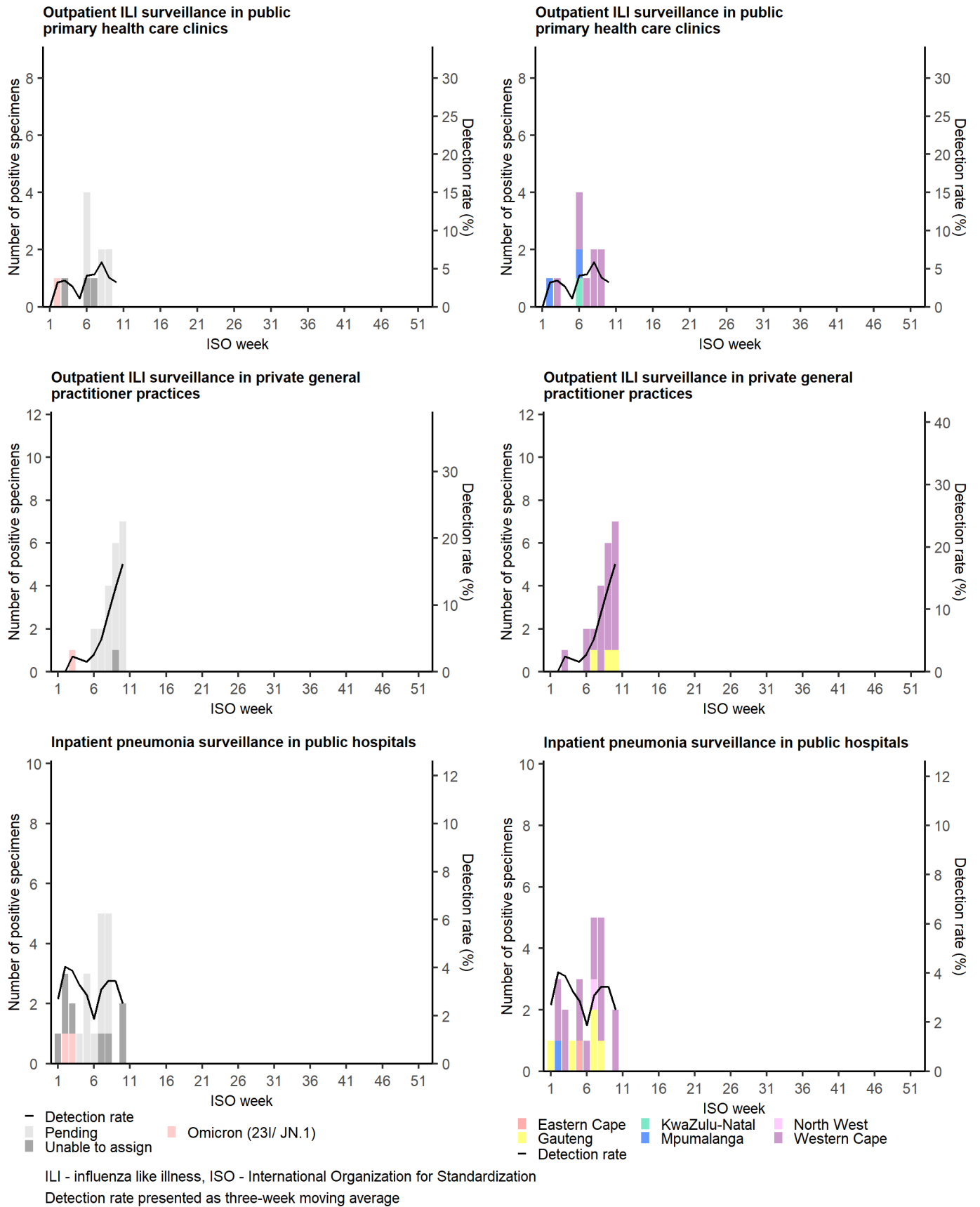
Figure 4: Number of laboratory-confirmed SARS-CoV-2 cases and detection rate by variant type (left) and province (right) in all ages, sentinel surveillance, South Africa, 2024-01-01 to 2024-03-10.
