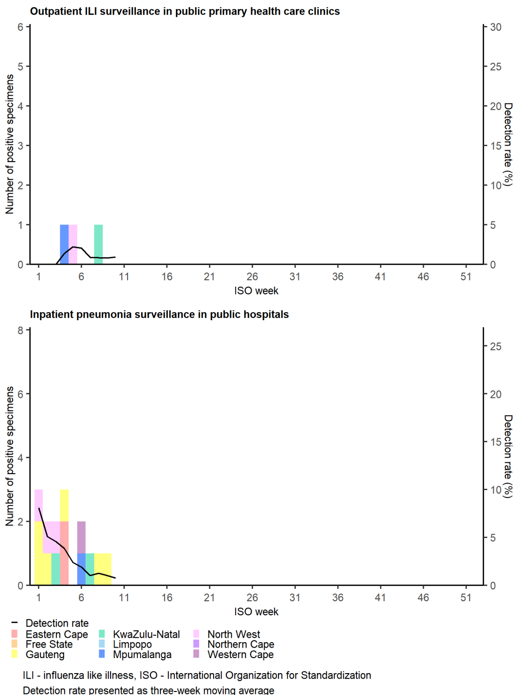
Figure 5: Number of laboratory-confirmed Bordetella pertussis cases and detection rate by province in all ages, sentinel surveillance, South Africa, 2024-01-01 to 2024-03-10.
