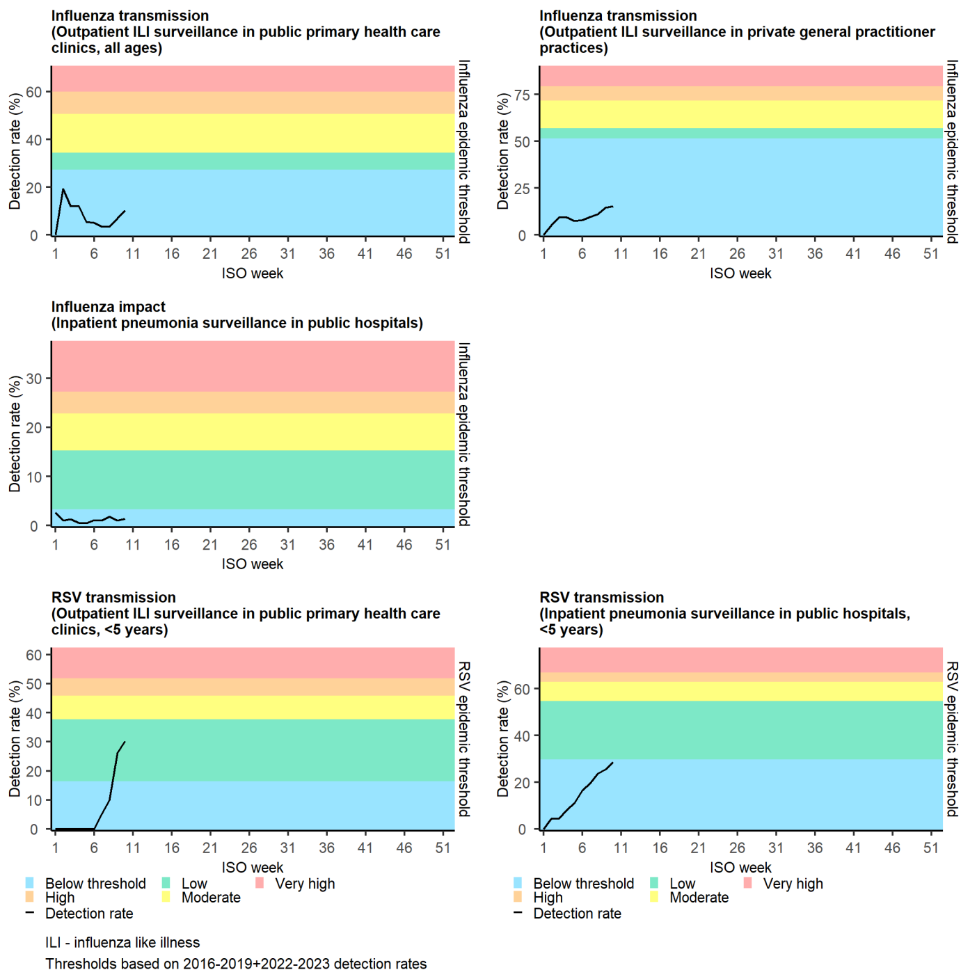
Figure 1: Influenza and respiratory syncytial virus (RSV) surveillance epidemic threshold summary, sentinel surveillance, South Africa, 2024-01-01 to 2024-03-10.
