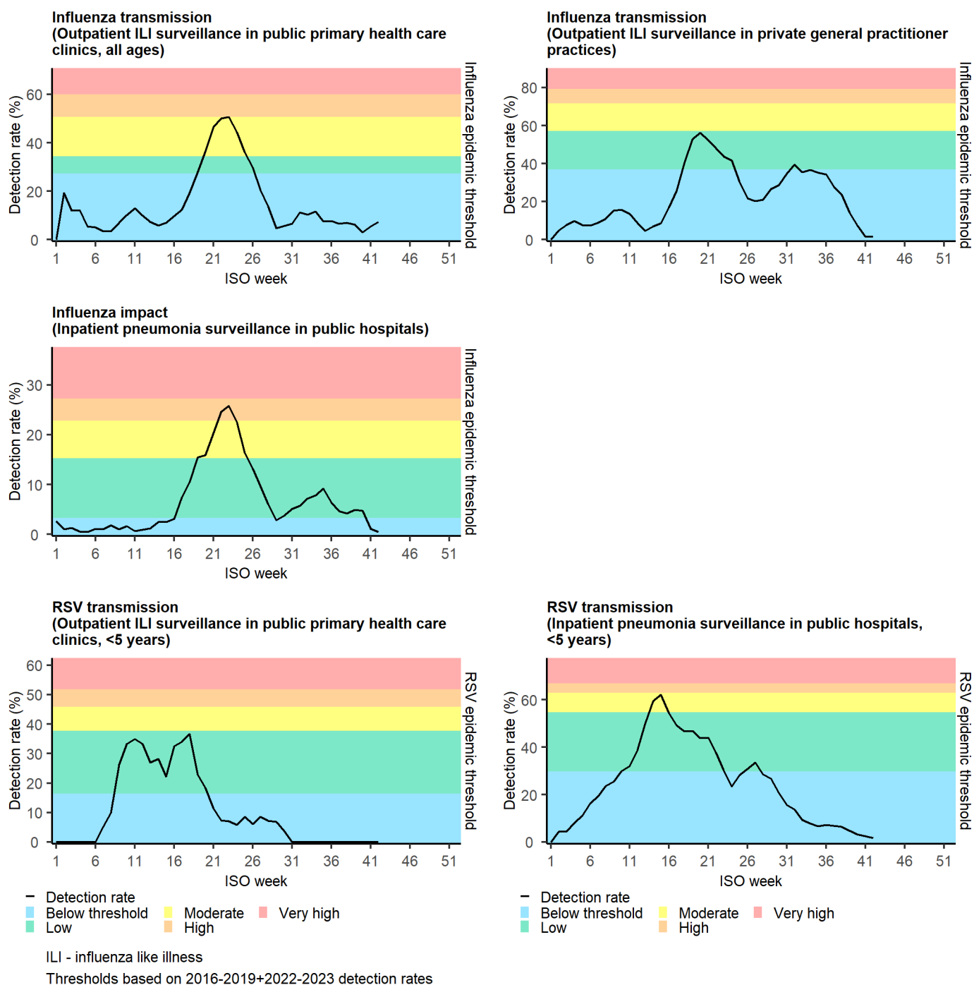
Figure 1: Influenza and respiratory syncytial virus (RSV) surveillance epidemic threshold summary, sentinel surveillance, South Africa, 01 January 2024 to 20 October 2024.
