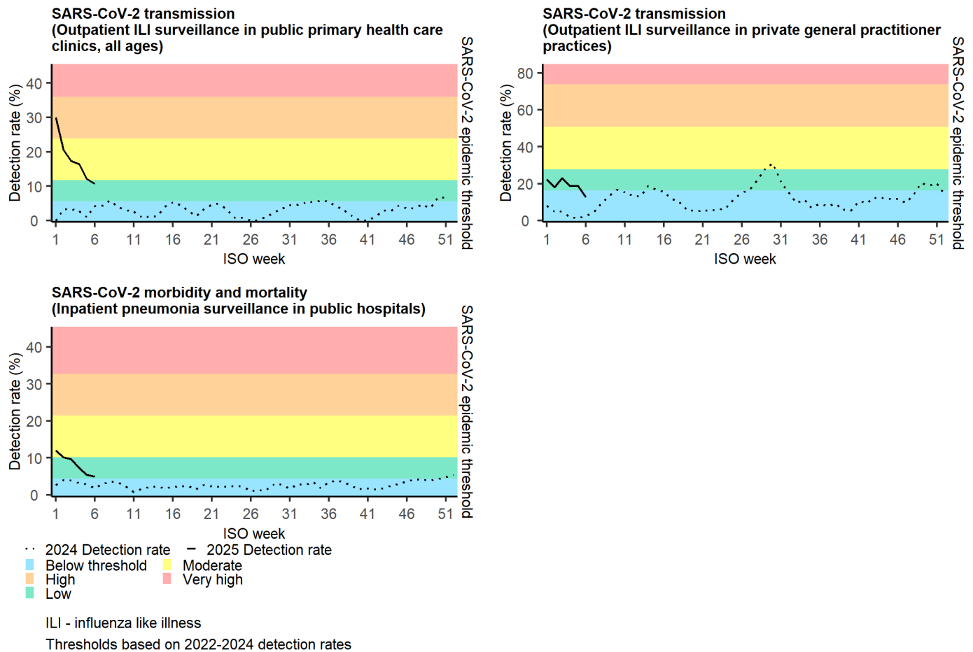
Figure 2: Severe acute respiratory syndrome coronavirus 2 (SARS-CoV-2) surveillance epidemic threshold summary, sentinel surveillance, South Africa, 30 December 2024 to 09 February 2025.
