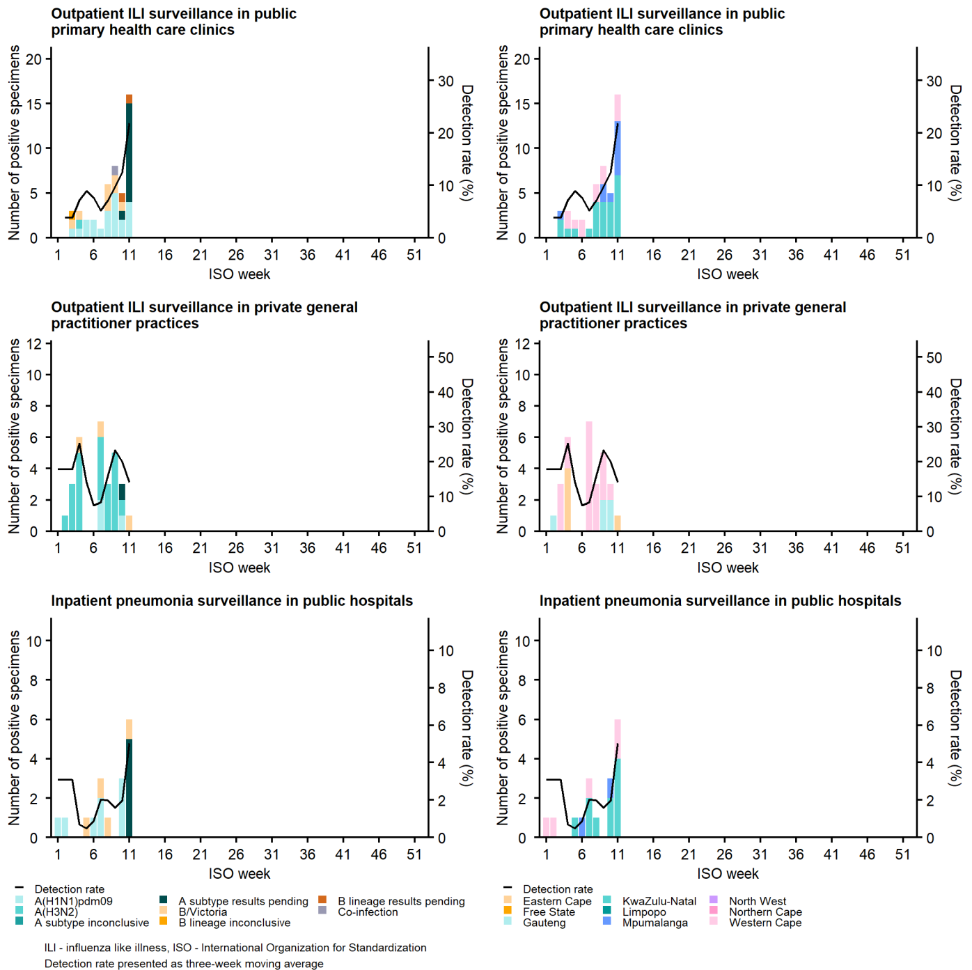
Figure 3: Number of laboratory-confirmed influenza cases and detection rate by subtype and lineage (left) and province (right) in all ages, sentinel surveillance, South Africa, 29 December 2025 to 15 March 2026.
